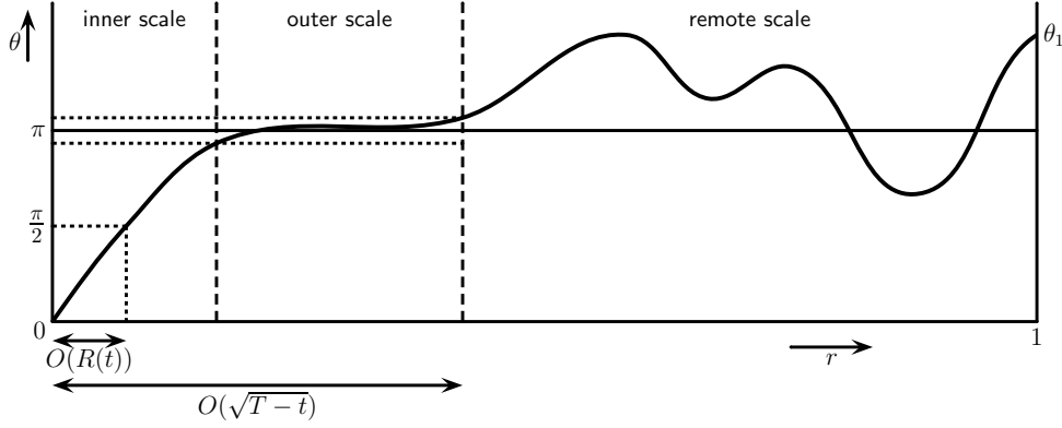
FIG. 3.1. Regions for asymptotic analysis
