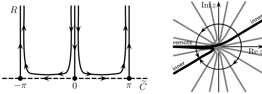
FIG. 5.1. Left: in the (\tilde{C}, R) phase plane the “stable manifold” of the blowup point acts as separatrix. Right: geometrically it is the boundary between a rotation over an angle \pi or -\pi .
