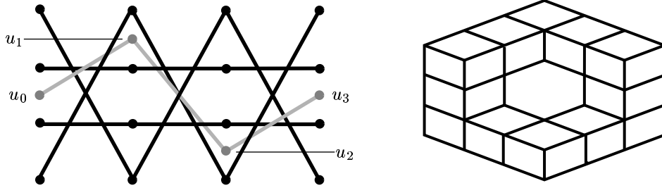
FIGURE 6. The braid of Example 2 and the associated configuration space N .
