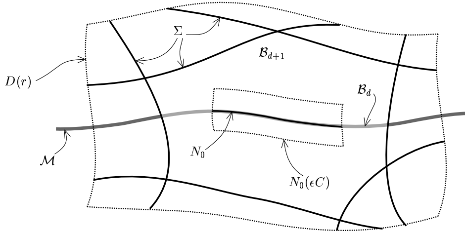
FIGURE 9. The rescaled flow acts on \mathcal{B}_{d+1} , the period d + 1 braid classes. The submanifold \mathcal{M} is a critical manifold of fixed points at \epsilon = 0 . Any appropriate isolating neighborhood N_0 in \mathcal{B}_d thickens to an isolating neighborhood in \mathcal{B}_{d+1} for \epsilon small.
