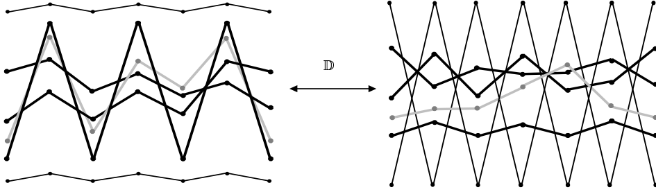
FIGURE 18. The augmentation of the braid from Lemma 50 [left] is the dual of the type III braid [right].
