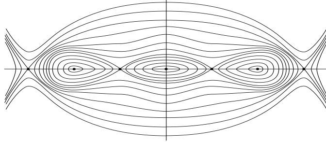
FIGURE 17. The integrable model in the (u, u_x) plane; there are centers at 0, \pm 2 and saddles at \pm 1, \pm 3 .
