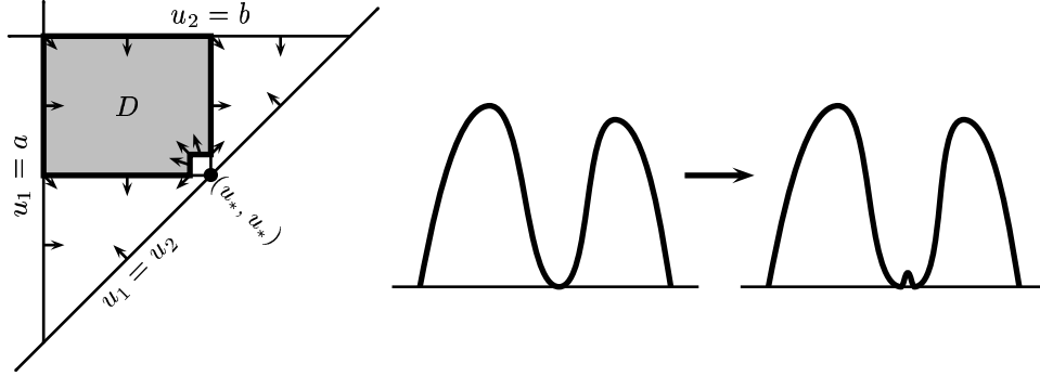
FIGURE 16. On the left the gradient of W_2 for the case of one saddle-focus equilibrium and compact boundary conditions. Clearly a saddle point is found in D . On the right the perturbation of one equilibrium to three equilibria.
