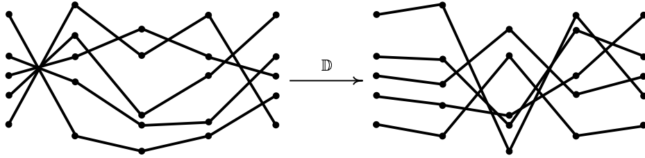
FIGURE 11. The topological action of \mathbb{D} .
