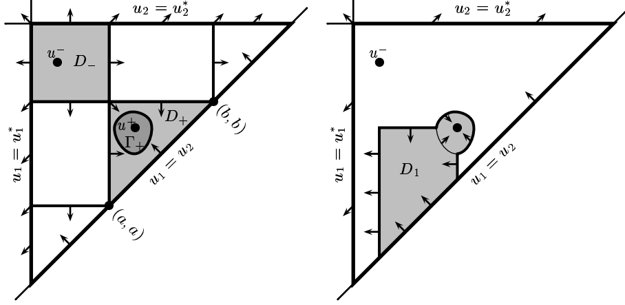
FIGURE 15. The gradient of W_2 for the case with two equilibria and dissipative boundary conditions. On the left, for E = 0 , the regions D_{\pm} with the maxima and minima u^{\pm} are depicted, as well as the superlevel set \Gamma^+ . On the right, for E \in (0, c_0) , the region D_1 , containing an index 1 point, is indicated.
