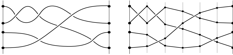
FIGURE 1. Examples of smooth [left] and discretized [right] positive braids on four strands. In a discretized isotopy, one slides the anchor points vertically.
