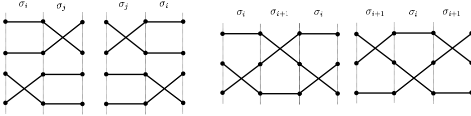
FIGURE 10. Relations in the braid group via discrete isotopy.
