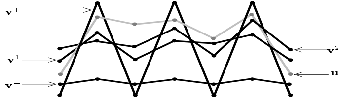
FIGURE 14. A representative braid class for the case I_E = \mathbb{R}^\pm : q = 1 , r = 4 , 2p = 6 .
