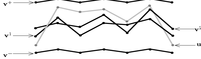
FIGURE 12. A representative braid class for the compact case: q = 1 , r = 4 , 2p = 6 .
