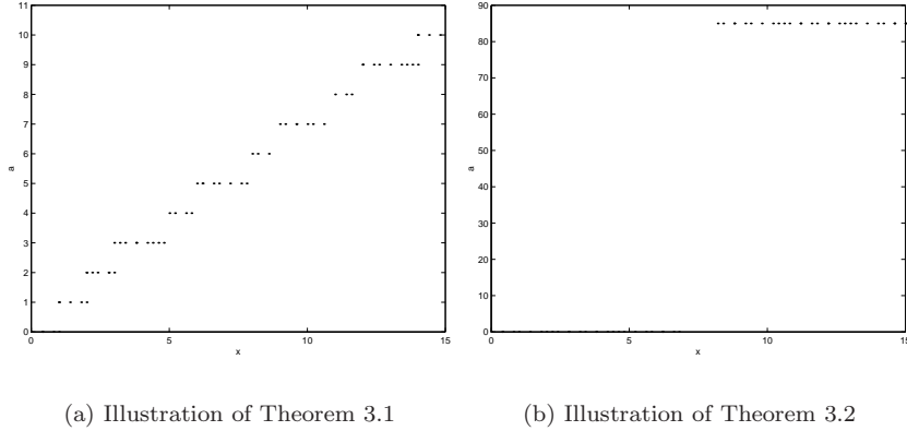
Figure 5: Numerical experiments to illustrate the structure of the optimal policy.
