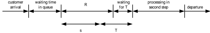
Figure 3: The service at step 1 is finished while computing resources are not available
