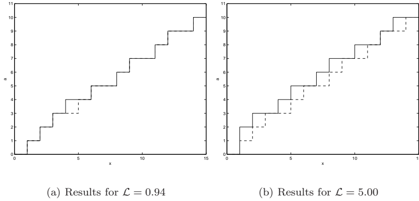
Figure 6: Numerical experiments to illustrate the effect of changing values of \mathcal{L} .
