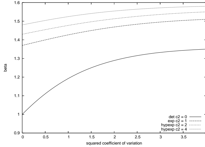
Figure 4: The time spent at station 1 for different distributions of R and T .
