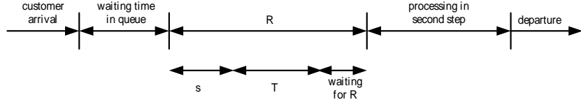
Figure 2: Computing resources are available before end of service at step 1
