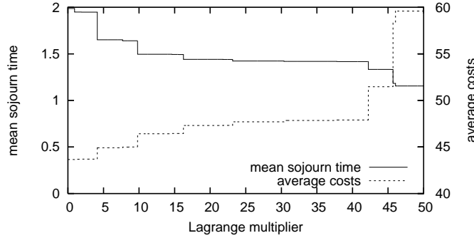
Figure 7: The average cost and the sojourn time as a function of the Lagrange multiplier.
