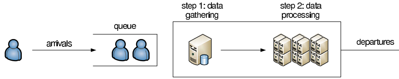
Figure 1: Service facility with two processing steps
