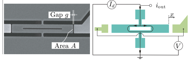
Figure 1. SEM micrograph and sketch of the MEMS resonator under study. A resistive output signal is measured by sending a current I_d through the resonator, which is electrostatically actuated by a voltage V , consisting of a biasing V_{\text{dc}} and a resonance-matched driving signal V_{\text{ac}} . The output is measured at the node labelled i_{\text{out}} . Area A is the frontal area, not visible in this top-view image, defined as material thickness times resonator width.
