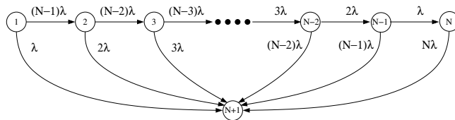
Figure 1: Two-hop multicopy protocol: transition diagram of the Markov chain for the number of copies.
