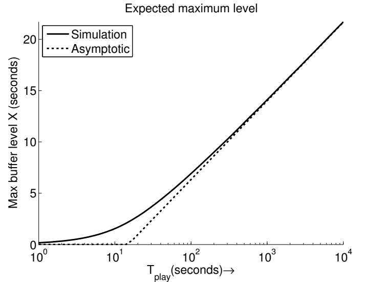
Fig. 6. Simulated and theoretical (asymptotic, see Equation (32)) expectation of the maximum level M^*(t) on logarithmic time-scale.
