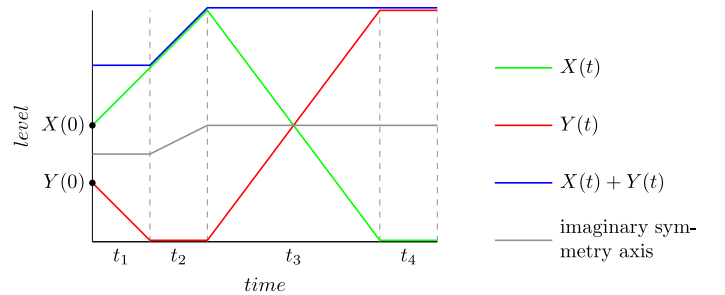
Fig. 3. Different behaviors of the stochastic processes.
