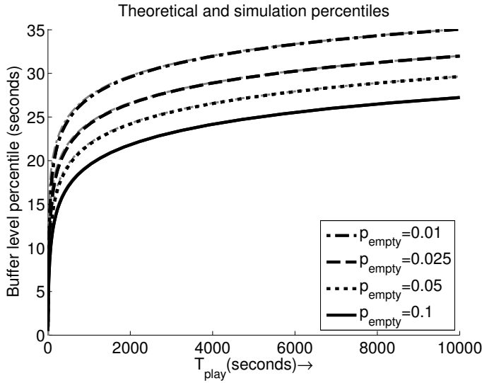
Fig. 7. Black lines represent simulation percentiles, gray lines represent theoretical asymptotic percentiles.
