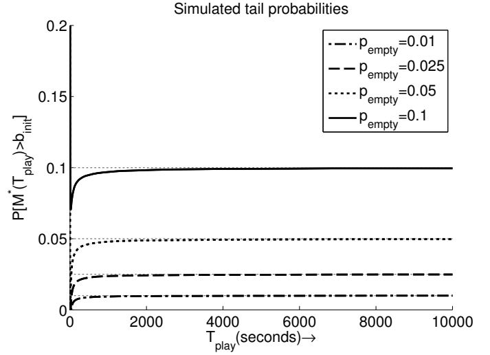
Fig. 5. Tail probabilities using empirical distribution based on simulation, evaluated on theoretical asymptotic percentiles.
