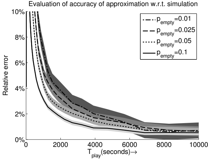
Fig. 4. Relative difference of buffer under-run probability to simulation. The gray bands around the lines are the 95% confidence intervals of the simulation.
