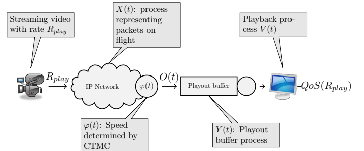
Fig. 1. Tandem of fluid buffers representing video streaming at rate R_{play} through an IP-network with variable output rate O(t) .
