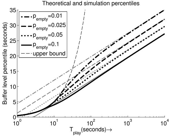
Fig. 8. Percentiles on logarithmic time scale. Black lines represent percentiles from simulation, gray lines represent theoretical asymptotic percentiles.
