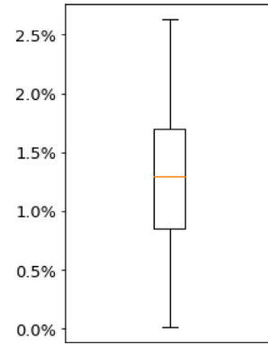
Fig. 6. Optimality gap in %.
