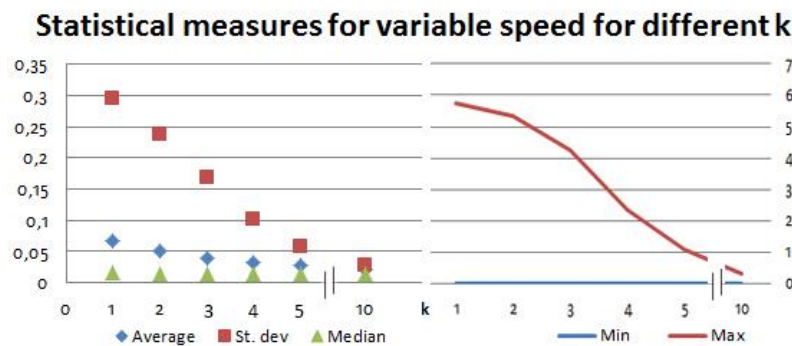
Figure 6 - Statistical measures for different k (number of historical tweets taken into account when calculating speed)
