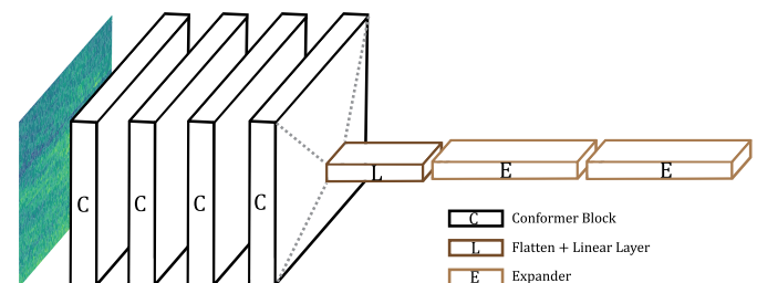
Fig. 1. The proposed architecture for the unsupervised framework. The framework starts with a Mel Spectrogram, followed by four Conformer Blocks (indicated in black), one flatten layer combined with a linear layer (indicated in brown), and finalized with an Expander (indicated in light brown).
