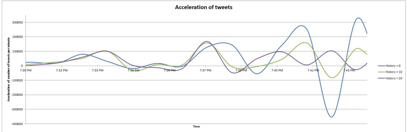
Figure 5. The acceleration of the number of tweets per second for different values of k (history) for #PrayforMexico on 20 March 2012.
