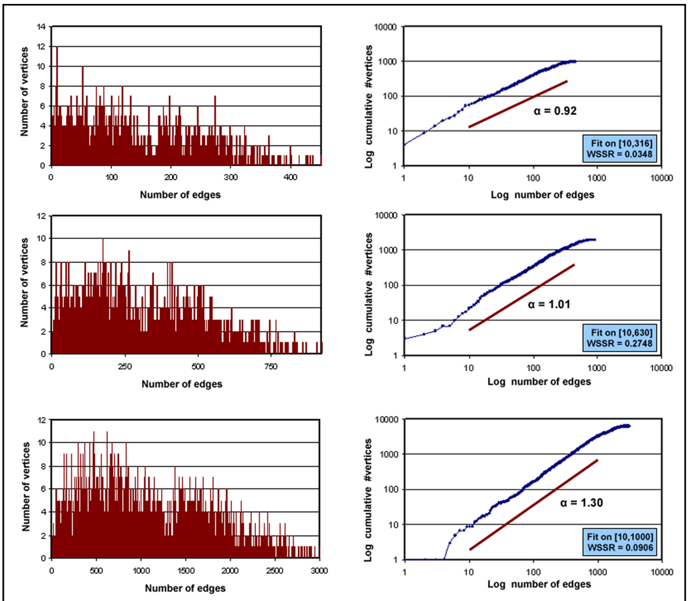
Figure 2. Degree distributions (left) of Kanji networks (top: Kyouiku, middle: JouYou, bottom: JIS X.02.08) show apparent featureless patterns. However, log-log plots of the cumulative networks of the same plots (right-hand side) show largely linear tendencies on the central part. The red line corresponds to both the exponent and the interval used for the specific network, the text directly below is the value of its exponent. The values in the inset boxes are fitting intervals and fitting errors. All fits were done with Fityk on Linux by the Levenberg-Marquardt method from random initial conditions.
