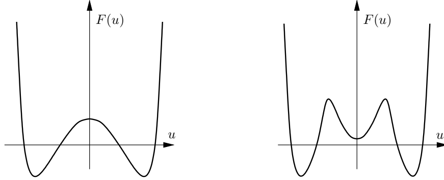
FIGURE 7. Swift-Hohenberg and modified Swift-Hohenberg potentials.
