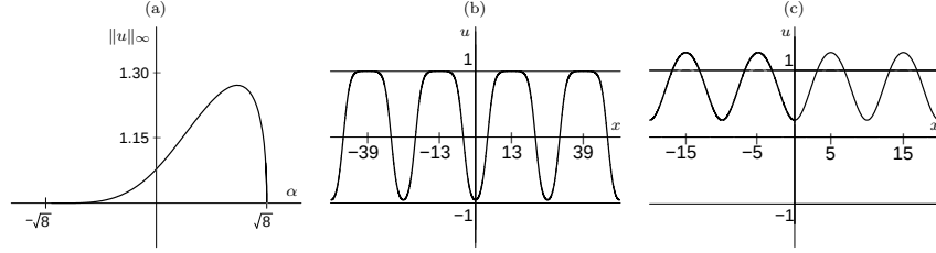
FIGURE 4. Reproduced from [13]. Bifurcation diagram for the solutions of the third type and corresponding solutions which are in the class \mathbf{u}_{1,1} . Solution (b) corresponds to \alpha = -1 and (c) to \alpha = 1 .
