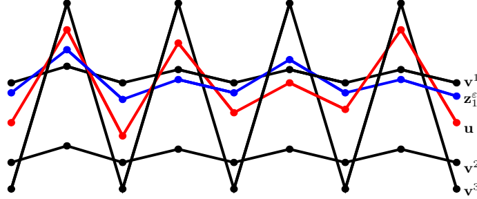
FIGURE 9. A representative of the braid class [\mathbf{u} \text{ rel } \mathbf{v}^\varepsilon] for p = 4, q = 3, p' = 1 and q' = 2 . If we leave out the strand \mathbf{z}_1^\varepsilon from the skeleton we get a representative of the braid class [\mathbf{u} \text{ rel } \mathbf{v}] .
