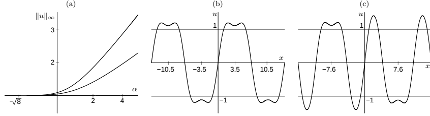
FIGURE 2. Reproduced from [13]. Bifurcation diagram for the solutions of the first type and corresponding solutions for \alpha = 1.5 . The number of monotone laps for the solution pictured at (b) is six and it intersects u_{\pm} two times. For solution (c) the number of monotone laps is ten and the crossing number with u_{\pm} is six.
