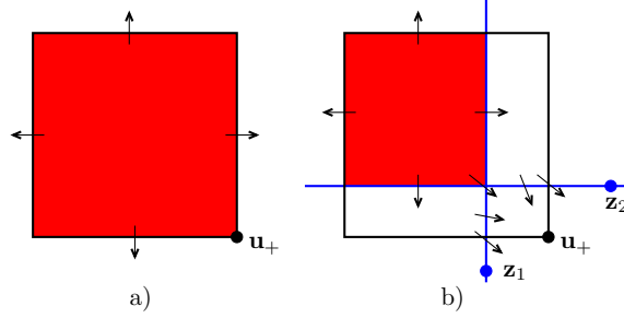
FIGURE 8. Figure (a) schematically shows the behavior of the vector field \mathcal{R} on the boundary of the improper braid class [\mathbf{u}]_\varepsilon \text{ rel } \mathbf{v} corresponding to the third type of solution. The strand \mathbf{u}_+ is a fixed point for the flow \Psi^t and some trajectories approach this point as t \rightarrow \infty . Figure (b) shows the behavior of the perturbed vector field on the boundary of the proper braid class [\mathbf{u}]_\varepsilon \text{ rel } \bar{\mathbf{v}} , where \bar{\mathbf{v}} = \mathbf{v} \cup \mathbf{z}_1 \cup \mathbf{z}_2 and \mathbf{z}_1, \mathbf{z}_2 are fixed strands for this perturbed vector field.
