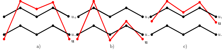
FIGURE 7. Representatives of the three different relative braid classes. A fixed point in the relative braid class defined by the depicted representative corresponds to the solution of a) type I, b) type II and c) type III. Braid classes (a) and (b) are proper, but (c) is not.
