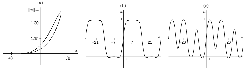
FIGURE 3. Reproduced from [13]. Bifurcation diagram for the solutions of the second type and corresponding solutions. Both solutions in (b) and (c) lie on the same bifurcation branch and have six monotone laps and cross u_{\pm} four times. The depicted solutions corresponds to the parameter value \alpha = -\frac{1}{10} .
