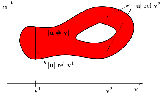
FIGURE 6. Relative braid classes and their fibers.
