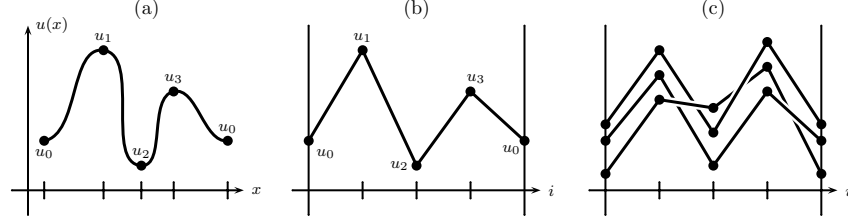
FIGURE 5. (a) A periodic function, (b) its piecewise linear graph, and (c) a braid consisting of 3 strands.
