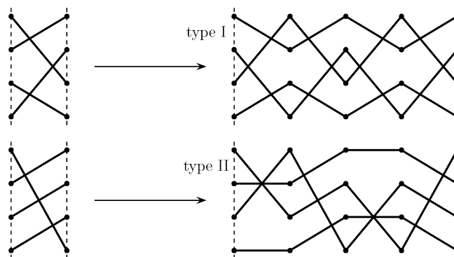
Fig. 1. Period-4 points lead to two possible braid classes. In the braid diagrams on the right one may think of all the crossings as being positive, i.e., the strand with the larger slope going on top.
