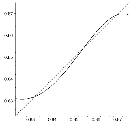
Fig. 12. One of the two trapping regions of the period-4 orbit. We choose \lambda so close to \lambda^* that the function is monotone between the three fixed points of F_\lambda^4 in the picture.
