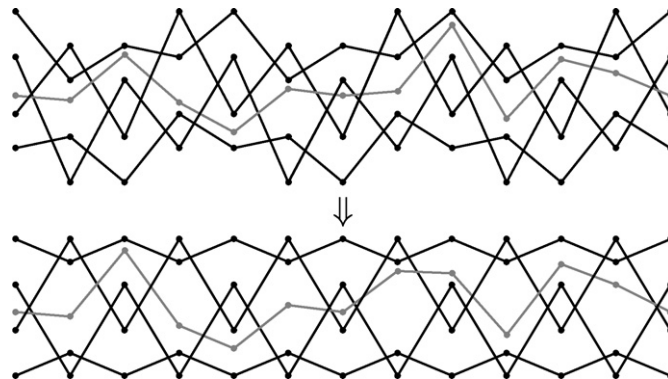
Fig. 10. Braid diagrams corresponding to \{\dots, a_0, a_1, a_2, a_3, a_4, a_5, a_6, \dots\} = \{\dots, 0, +1, +1, 0, -1, +1, 0, \dots\} . At the top is a generic non-symmetric situation, while at the bottom the skeleton is deformed into a symmetric one, which has the same topological information and has the advantage that it is a lot easier to survey. The homotopy type of this braid class is the pointed space (S^2, \text{pt}) .
