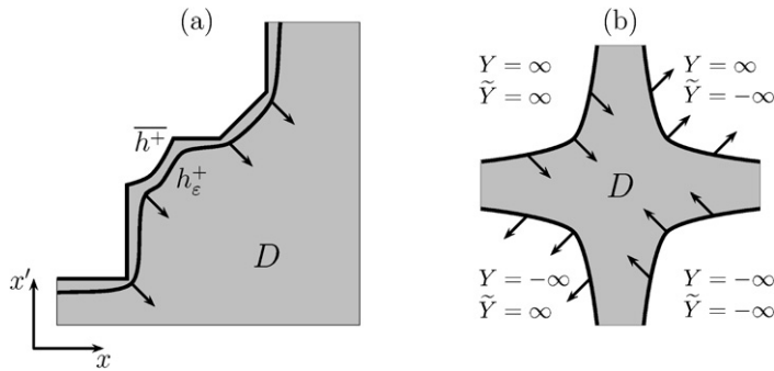
Fig. 14. (a) The northwest corner and its \varepsilon -approximation with the direction of the flow. (b) Cartoon of the four pieces of boundary of the domain.
