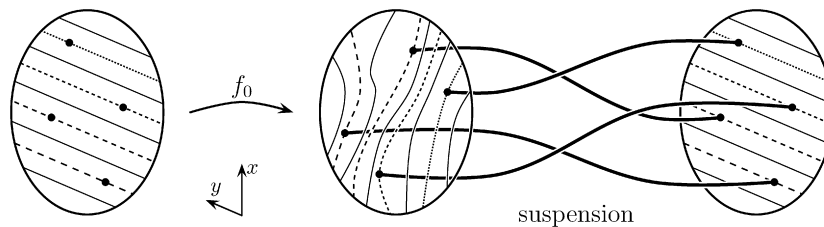
Fig. 3. The map f_0 is orientation preserving and has the twist property, hence the suspension looks like a distorted rotation, which leads to a positive braid.
