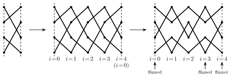
Fig. 8. Starting from an ordering of the points (x^0, x^1, x^2, x^3) on the left ( f permutes the ordered points), one uses four iterates (middle) and then applies the flip (i.e., inverting the order at the zeroth and third coordinates) to obtain the braid diagram on the right.
