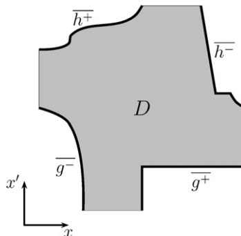
Fig. 13. The domain D of the functions Y_f and \tilde{Y}_f for a twist diffeomorphism f .
