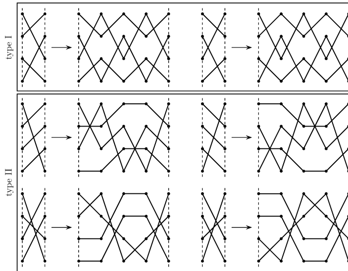
Fig. 9. The six period-4 orbits and their corresponding braid diagrams.
