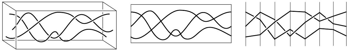
Fig. 4. Example of a braid on three strands. [left] A braid with all crossings positive (bottom over top), [middle] its 2-d projection, and [right] the associated piecewise linear braid diagram, a discretized braid. Its braid word is \sigma_2\sigma_1\sigma_2\sigma_1^2\sigma_2^2 .
