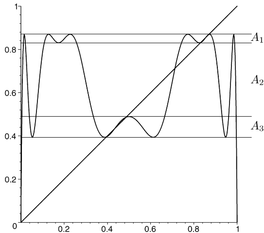
Fig. 11. The graph of the fourth power of the quadratic map. The parameter \lambda is set to \lambda^* + 0.04 . The intervals A_1 , A_2 and A_3 (bounded by the extrema) are indicated.
