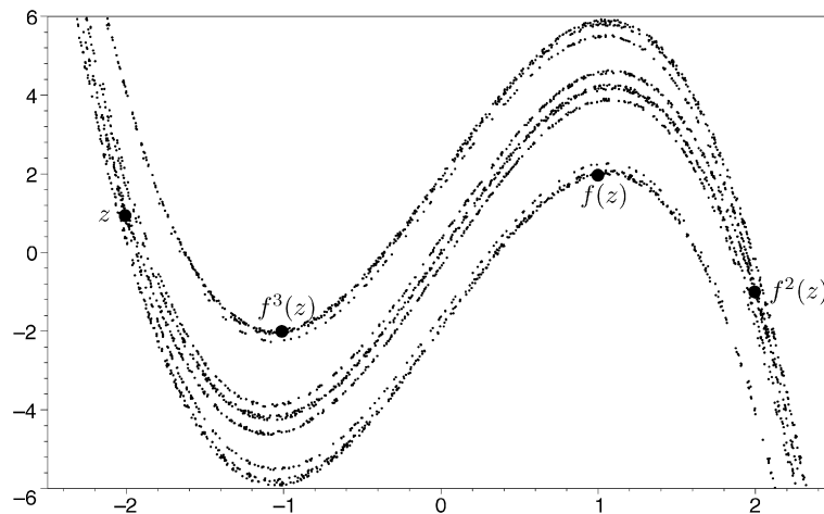
Fig. 2. Orbits of the map f(x, y) = (y, x + \frac{17}{3}y - \frac{5}{3}y^3) . A period-4 orbit of type I is indicated by the large dots.
