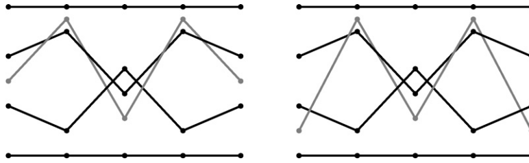
Fig. 6. Two bounded braids with the same skeleton (black lines); the free strand is the gray line. The braid on the left is improper (one can deform the free strand to one of the strands of the skeleton), the one on the right is proper.
