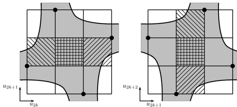
Fig. 15. The dots represent the points (v_i^\alpha, v_{i+1}^\alpha) \in D_i , \alpha = 1, 2, 3, 4 , for even i (left) and odd i (right). The domain D_i is indicated in gray. The projections of the unrestricted braid classes onto the (u_i, u_{i+1}) -plane are hatched. Of the four boundaries of D_i only two can intersect the unrestricted braid classes.
