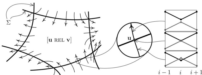
Fig. 5. A schematic picture of a parabolic flow on a (bounded and proper) braid class.
