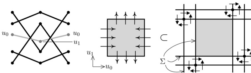
Fig. 7. In the relative braid on the left black lines denote the skeleton and gray lines the free strand. In the middle its configuration space is shown and the direction of the parabolic flow on the boundary is indicated. On the right we see how the configuration space is positioned with respect to the stationary points of the skeleton, represented by the four dots.
