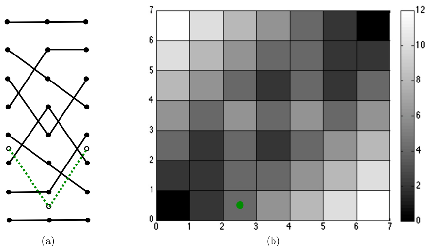
Fig. 2.2. (a) The skeleton \mathbf{v} (solid lines) and a free strand \mathbf{u} (dashed lines) with intersection number \iota(\mathbf{u}, \mathbf{v}) = 4 . (b) The (cubical) space of bounded configurations of free strands \mathbf{u}' . The free strand \mathbf{u} depicted in (a) has coordinates (2.5, 0.5) in (b). The grey-scale specifies the intersection number \iota(\mathbf{u}', \mathbf{v}) .
