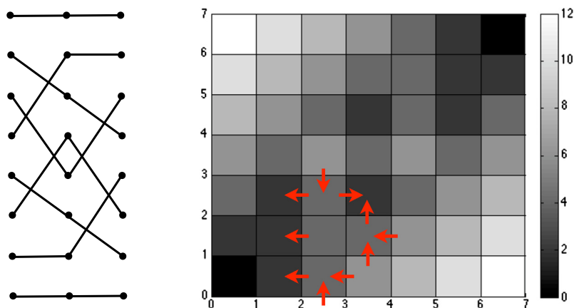
Fig. 2.4. On the boundary of each connected component of a discrete section of a relative braid class the direction of the flow can be determined on the basis of the total intersection number indicated by the grey-scale.
