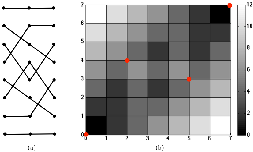
Fig. 2.3. (a) The skeleton \mathbf{v} and (b) the (cubical) space of all configurations of a free strand \mathbf{u} , shaded by intersection number \iota(\mathbf{u}, \mathbf{v}) . There are four closed skeletal strands at (0, 0) , (2, 4) , (5, 3) , and (7, 7) . These are labeled with red dots in (b). The bounded discrete relative braid class components are those cubical regions consisting of cubes with the same crossing number which are connected by codimension-1 faces. Since a relative braid class component labeled with a red dot contains a free strand configuration that may be collapsed onto a skeletal strand, these components are not proper. The remaining depicted relative braid class components are proper and bounded. (For interpretation of the references to color, the reader is referred to the web version of this article.)
