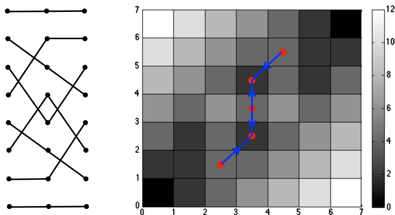
Fig. 3.1. On the basis of the Conley indices the existence of the indicated orbit structure can be concluded for any parabolic flow (1.3) that fixes the skeleton on the left. The red dots indicate invariant sets, not necessarily stationary points. (For interpretation of the references to color in this figure legend, the reader is referred to the web version of this article.)
