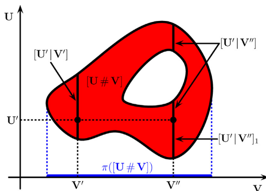
Fig. 2.1. A relative braid class [U \# V] in red and its projection \pi([U \# V]) in blue. Two fibers are indicated, one consisting of a single connected component, the other consisting of two components [U' | V'']_1 and [U' | V'']_2 . (For interpretation of the references to color in this figure legend, the reader is referred to the web version of this article.)
