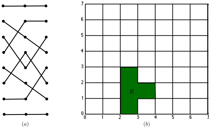
Fig. 1.2. The skeleton \mathbf{v} and the cubical relative braid class \mathcal{B} corresponding the four representatives in Fig. 1.1, depicted in the space of all discrete configurations of the free strand.
