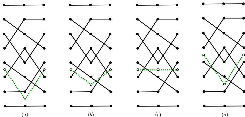
Fig. 1.1. (a) A free strand \mathbf{u} (dashed lines) relative to the skeleton \mathbf{v} (solid lines). (b), (c), (d) Additional free strand configurations within the same relative braid class \mathcal{B} = [\mathbf{u}|\mathbf{v}] , which is depicted in Fig. 1.2.
