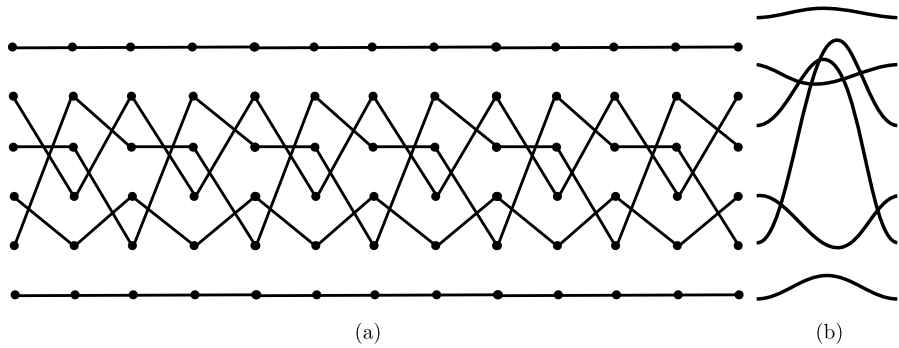
Fig. 5.1. (a) A discretized skeleton \mathbf{v} which is a 6-fold repetition of the continuous braid in (b).
