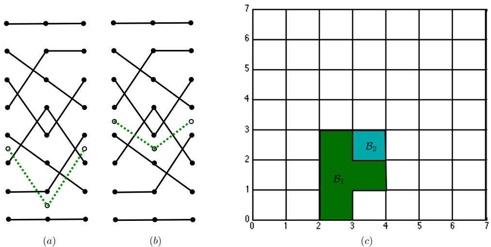
Fig. 1.3. Representatives \mathbf{u}_1 in (a) and \mathbf{u}_2 in (b) of braid classes \mathcal{B}_1 and \mathcal{B}_2 , respectively. Both braid classes are depicted in (c).
