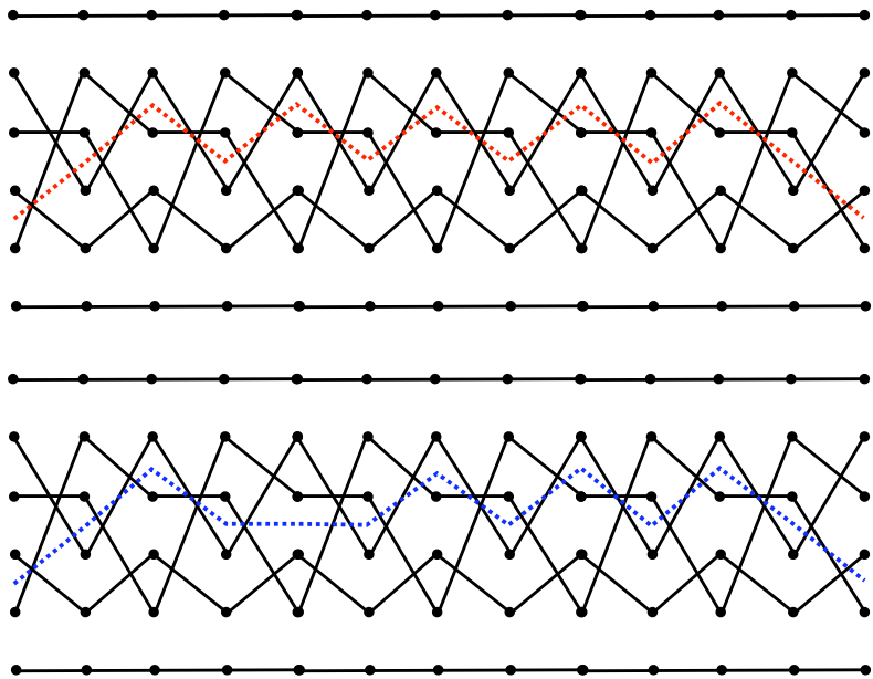
Fig. 5.2. Two relative braids, top: (dashed) free strand \mathbf{u}_1 , bottom: (dashed) free strand \mathbf{u}_2 .
